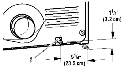
1. 3/8 in. NPT dryer pipe
