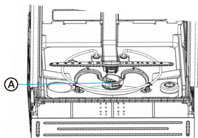
Ⓐ Filter Location
