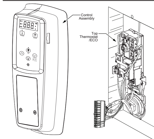
Figure 21 - Control Assembly
