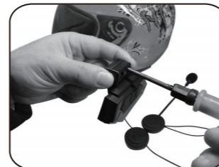
Fig.2 Move the clip and align it on the left side of the helmet Edge in.
