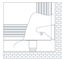
Anti-tip device for 36 inch
