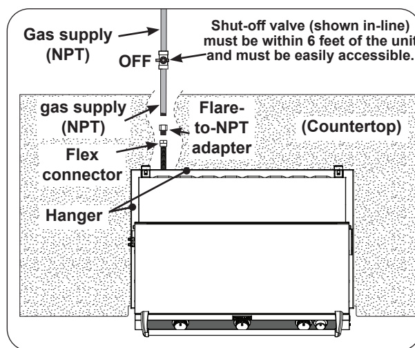
Fig. 30-2 Household LP & Nat. gas diagram
