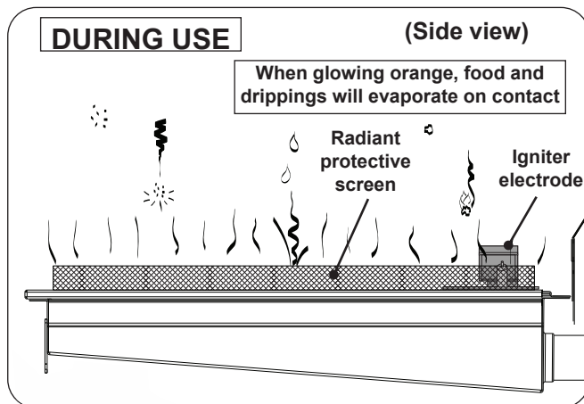
Fig. 43-3 Infrared burner - DURING USE
