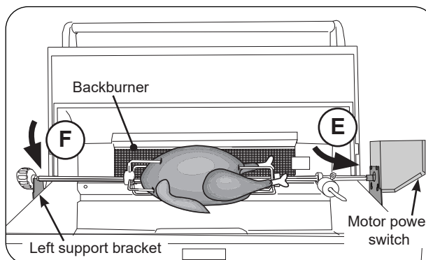
Fig. 42-4 Attach Rotisserie rod to motor
