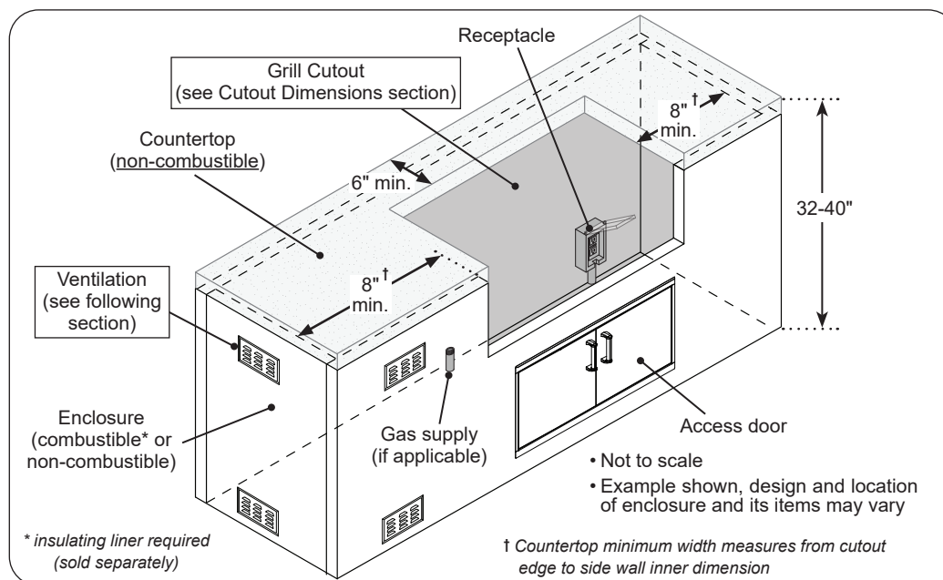
Fig. 11-1 Enclosure specifications
