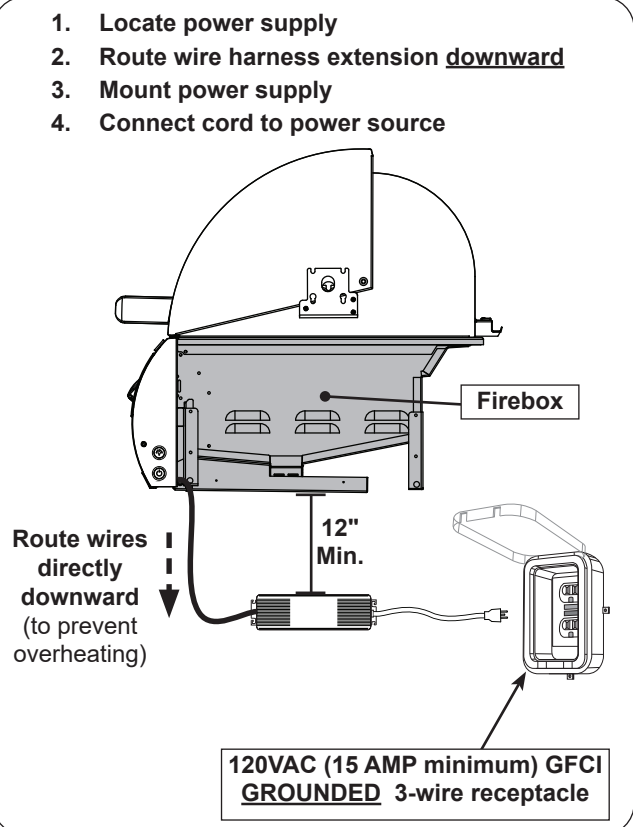
Fig. 29-3 Electrical installation
