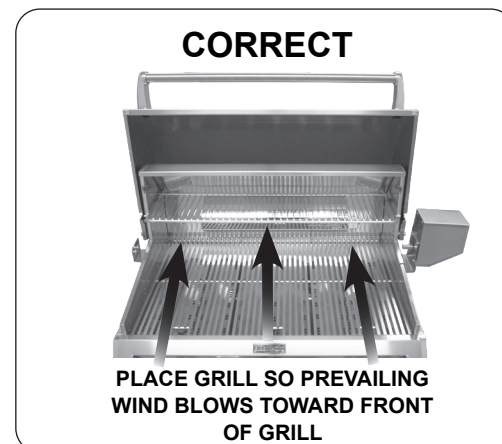
Fig. 19-3 Airflow direction - CORRECT
