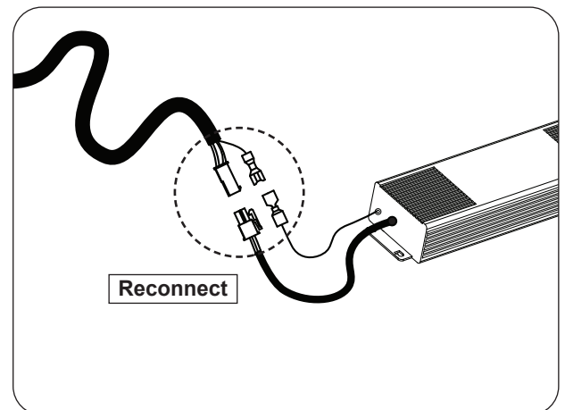
Fig. 29-2 Reconnect harness
