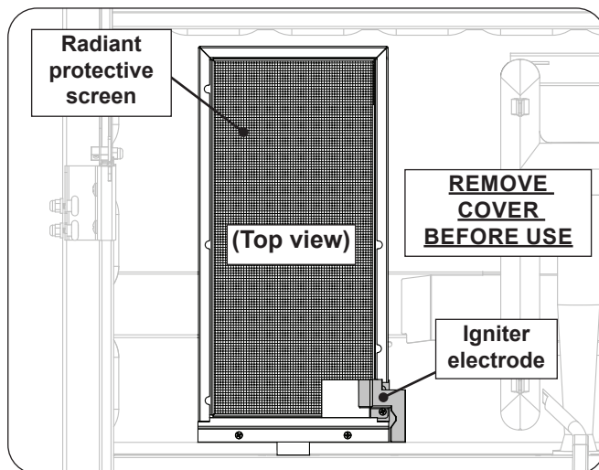
Fig. 43-1 Infrared burner overview
