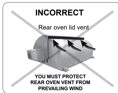
Fig. 19-4 Airflow direction - INCORRECT
