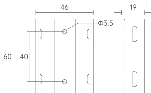
Plastic Bracket
