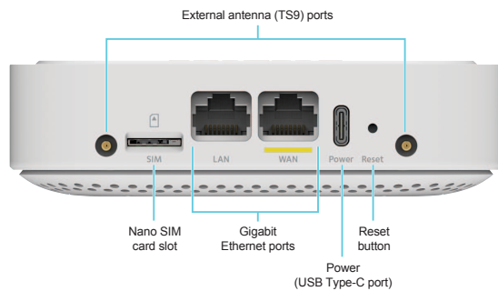
Figure 3. Back Panel
