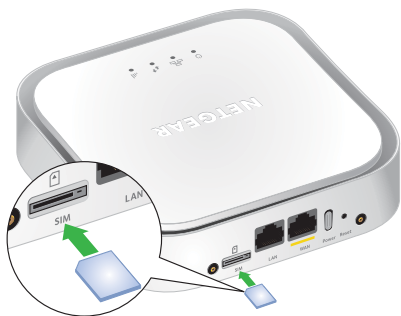
Figure 2. Installing the nano SIM card
