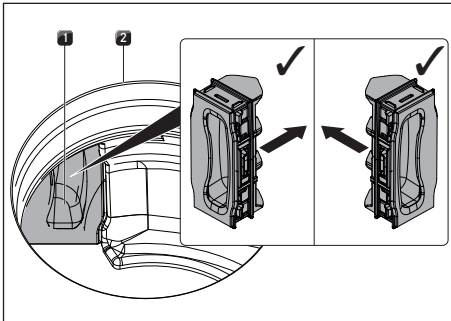
Fig. 8.10 Inserting the filter replacement cover
