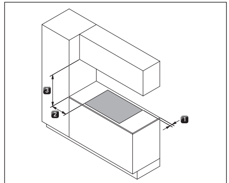
Fig. 10.3 Required clearance distances
