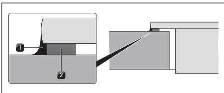
Fig. 10.24 Sealing tape in the case of surface mounting
