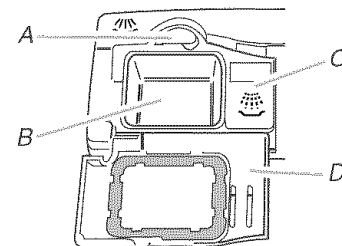
A. Cover latch B. Main Wash section C. Pre-Wash section D. Cover
