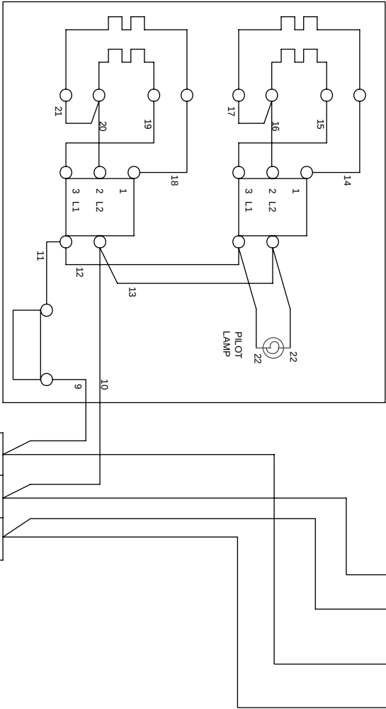
OVEN WIRING DIAGRAM.
