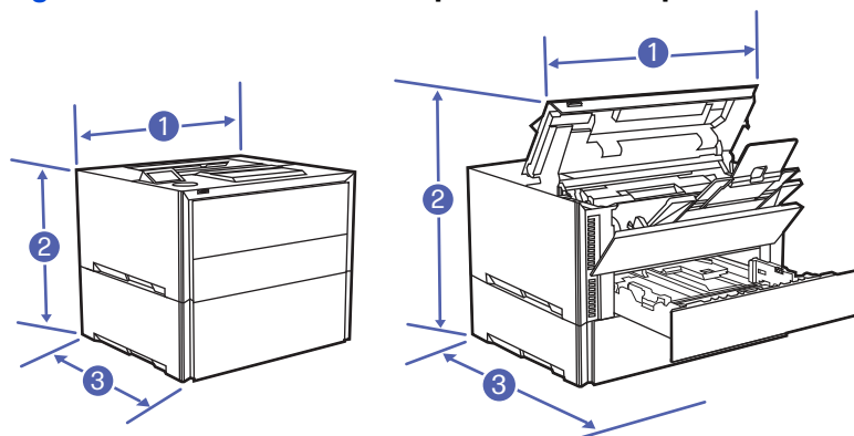
Figure 1-10 Dimensions for the printer with the optional 550-sheet tray
