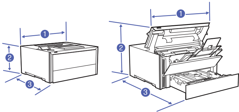
Figure 1-9 Dimensions
