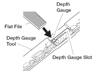
Figure 25 - Depth Gauge Tool On Chain
