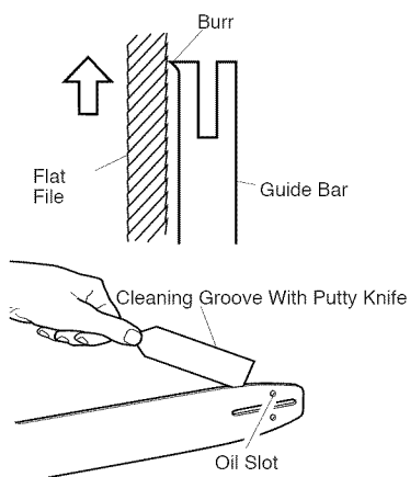
Figure 22 - Guide Bar Maintenance
