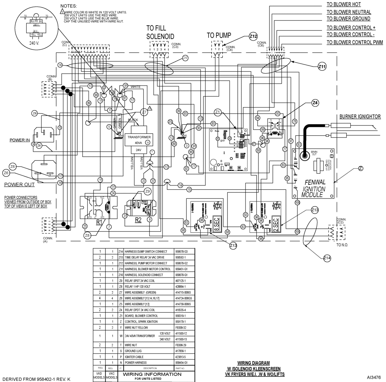
Power Supply Box (Before 12/1/12) - VK Fryer with basket lifts and Kleenscreen
