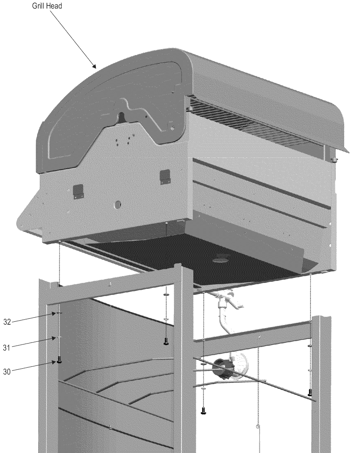
30 1/4-20x1/2" screws Qty. 4
