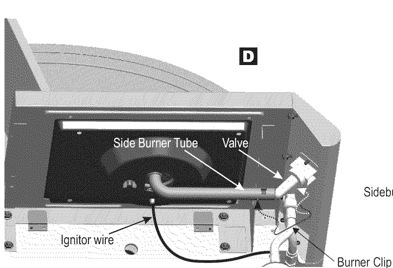
Correctly assembled burner-to-valve engagement
