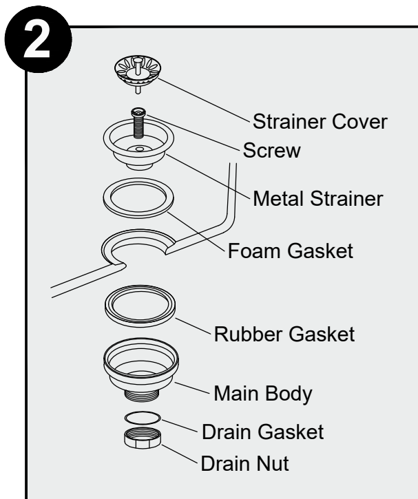
Disassemble the strainer
