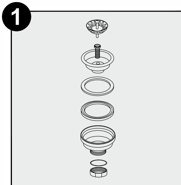
Disassemble the strainer
