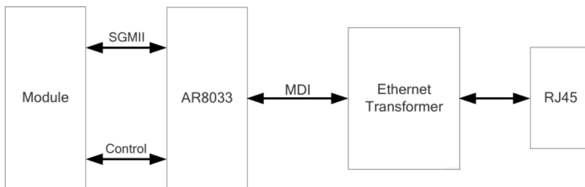
Figure 22 Simplified Block Diagram for Ethernet Application
