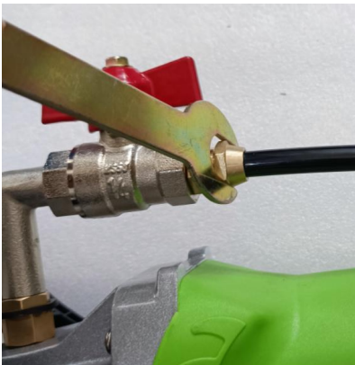
3. Install water pipe joints, Lock with a wrench.
