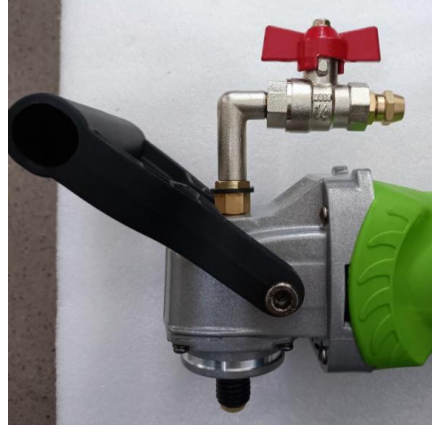
2. Install water valve
