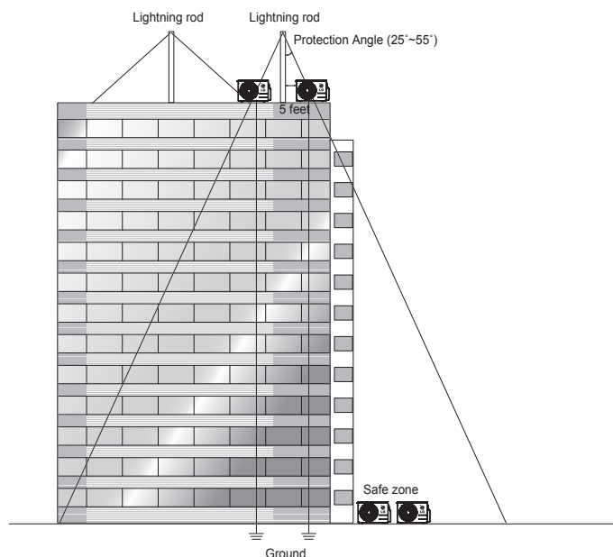
Figure 44: Lightning Protection Diagram.
