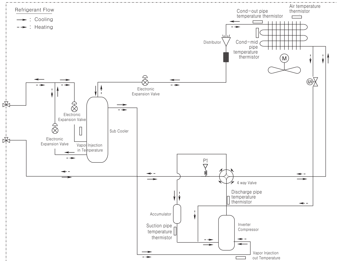
Figure 23: LUU420HHV, LUU480HHV Refrigerant Flow Diagram.
