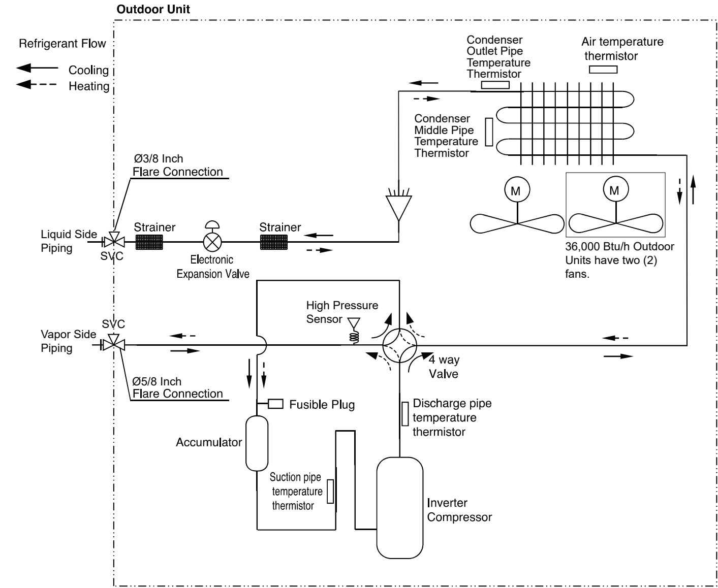
Figure 22: LUU180HHV, LUU240HHV, LUU360HHV Refrigerant Flow Diagram.
