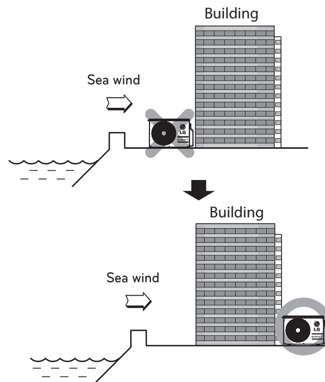
Figure 46: Placement Using Building as Shield.
