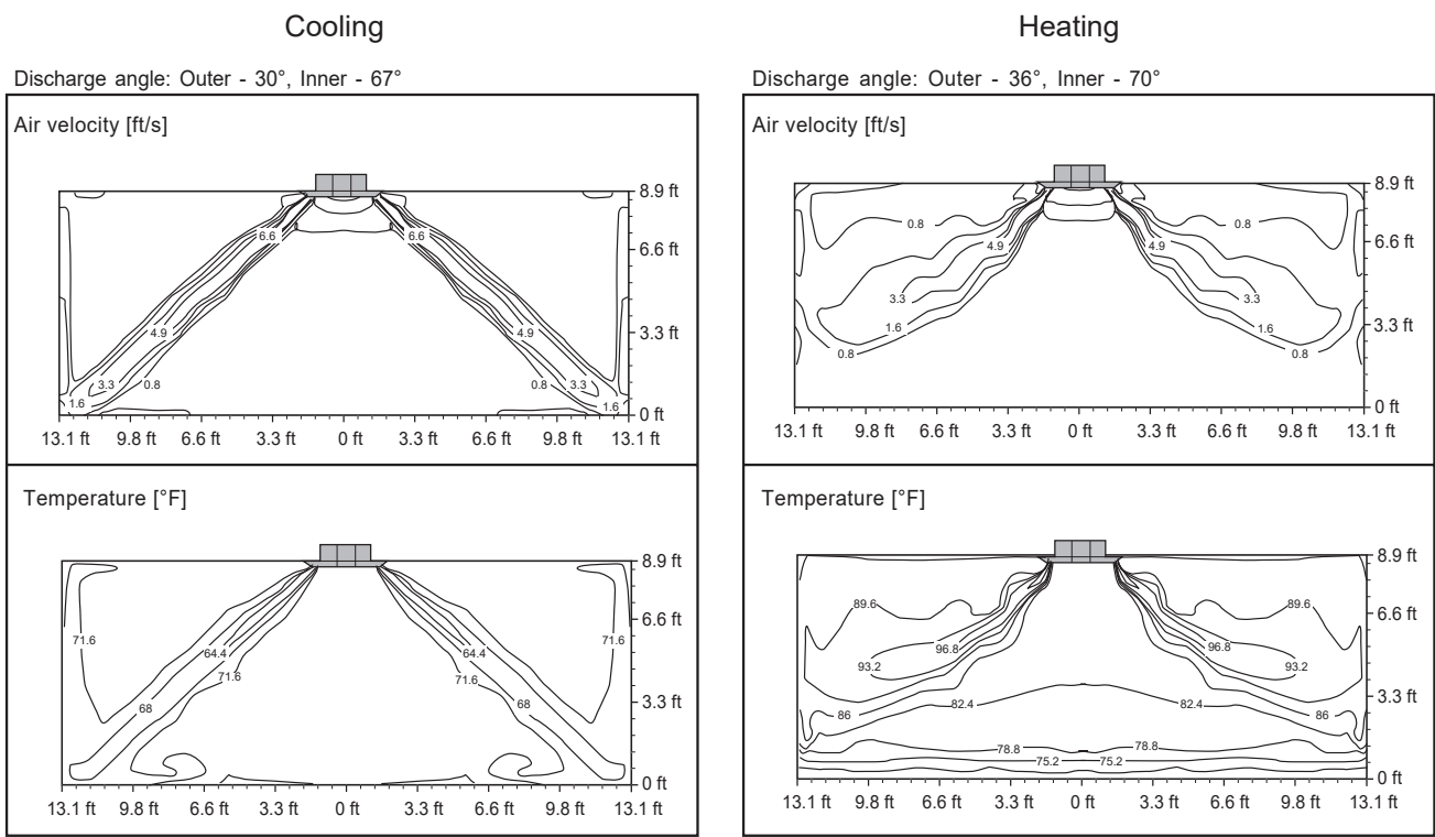
Figure 35: LCN249HV Air Velocity and Temperature Distribution Charts.
