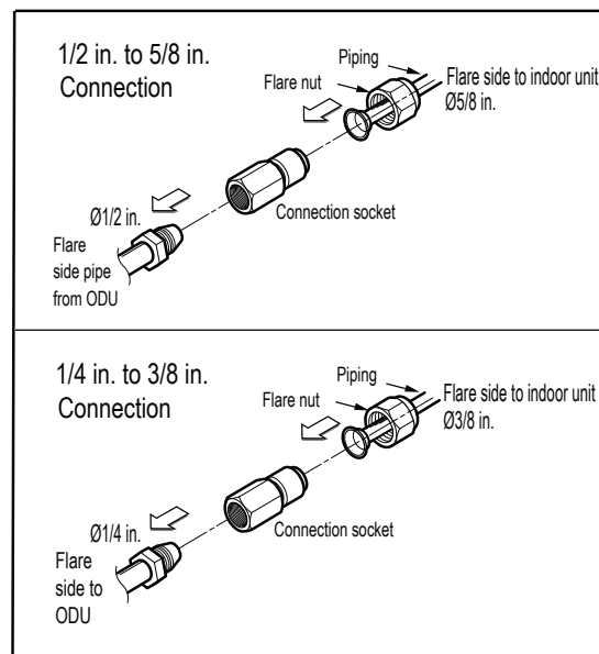
Figure 19: LCN188HV4 Refrigerant Pipe Connections.
