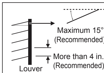
Figure 48: Louver Recommendations.
