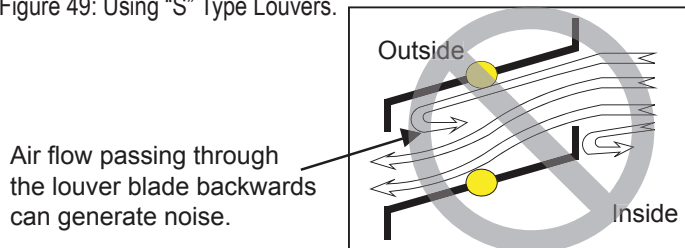
Figure 49: Using “S” Type Louvers.
