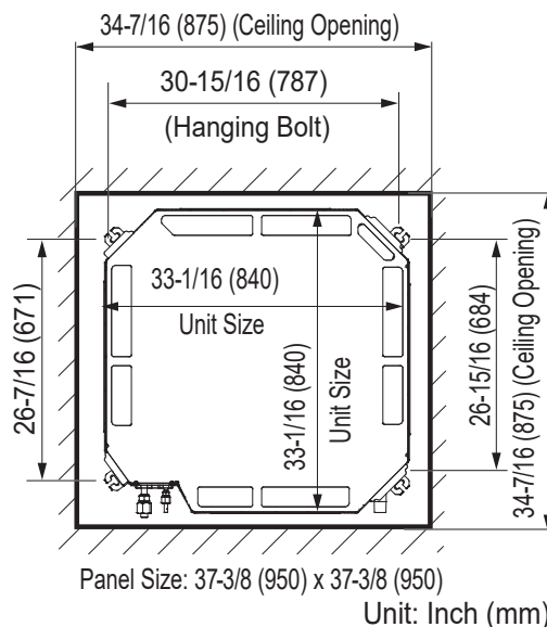
Figure 42: 3 x 3 Cassette Ceiling Opening Dimensions and Bolt Locations.
