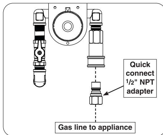
Fig. 2-4 Connect to gas line
