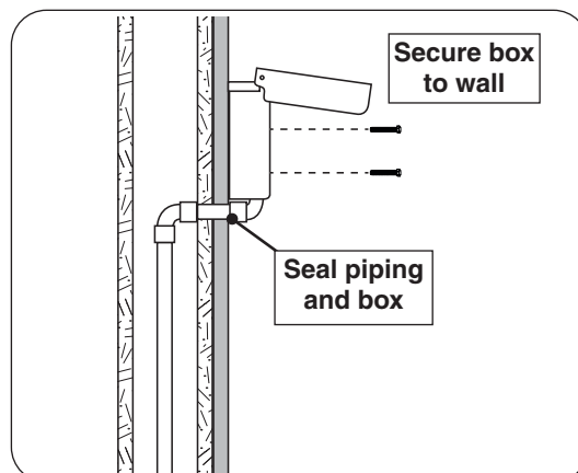
Fig. 2-3 Install stainless steel box
