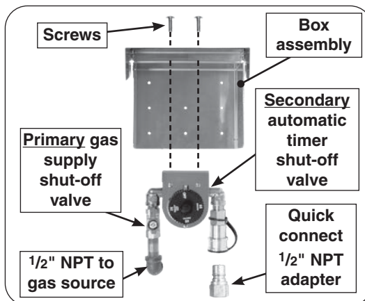
Fig. 1-1 Parts list
