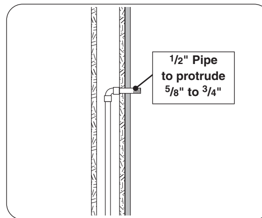
Fig. 1-2 Piping detail
