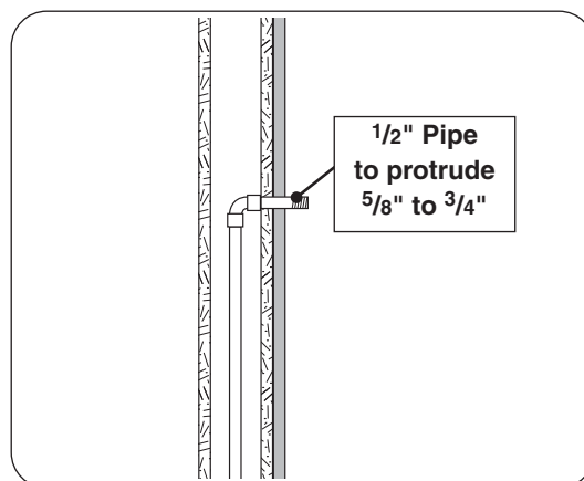
Fig. 2-1 Route gas supply
