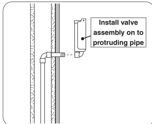
Fig. 2-2 Install valve assembly
