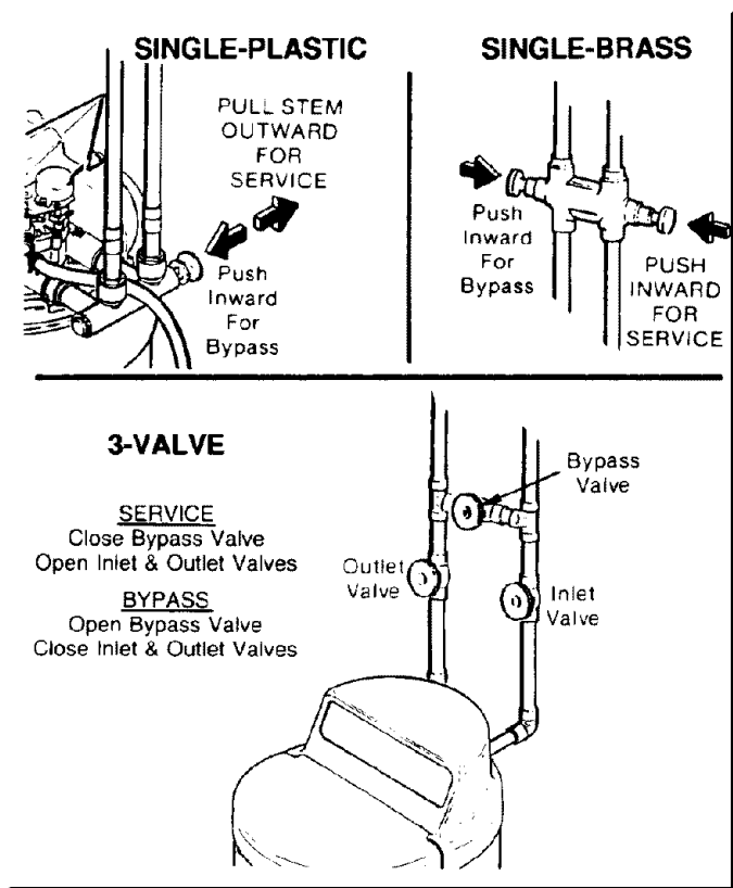
FIG. 12 BYPASS VALVES
