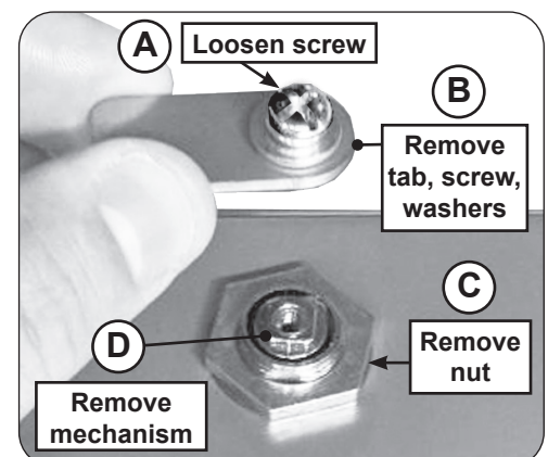
Fig. 4-5 Locking / unlocking
