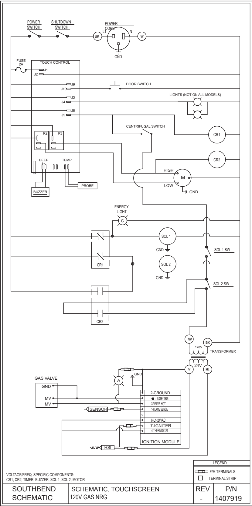
Figure 36 Wiring Diagram for 120 Volt Gas NRG Touchscreen Models
