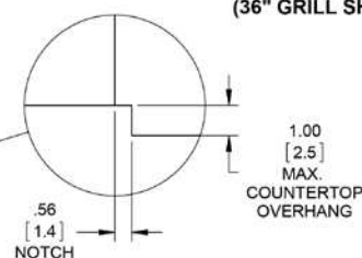
TYPICAL ISLAND INSTALLATION (36" GRILL SHOWN)
