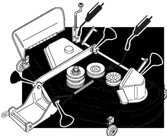
Figure 16. Mower Lubrication
