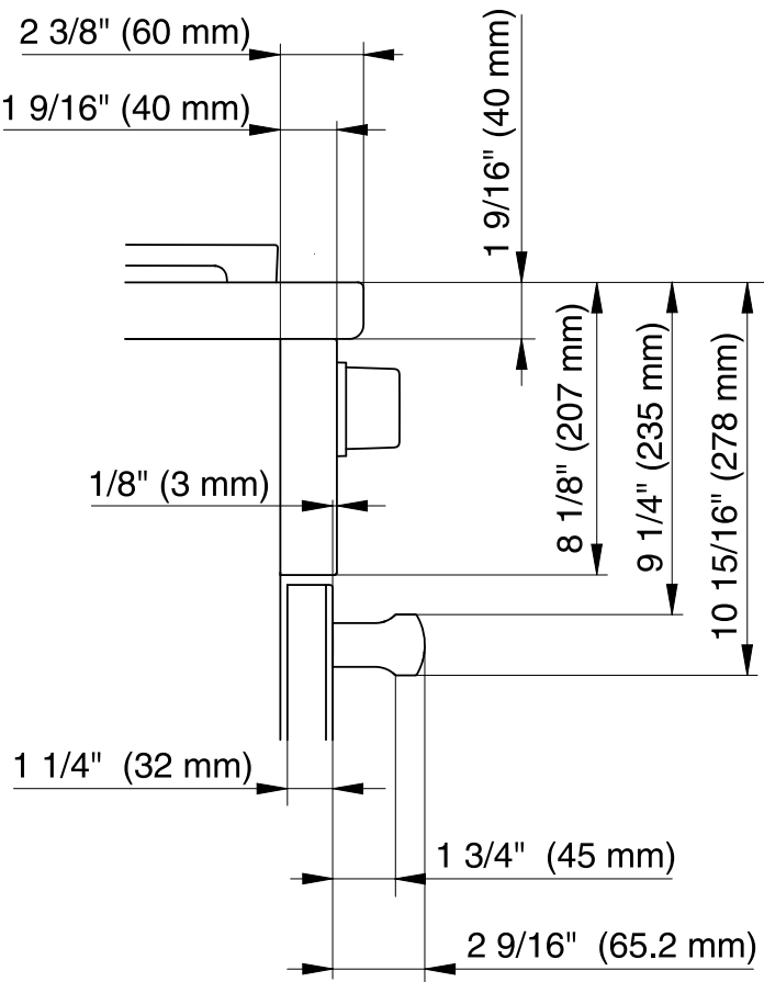
Detailed front side view of HR 1956-3 DF
