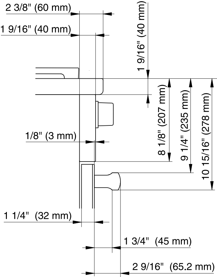
Detailed front side view of HR 1955-3 DF
