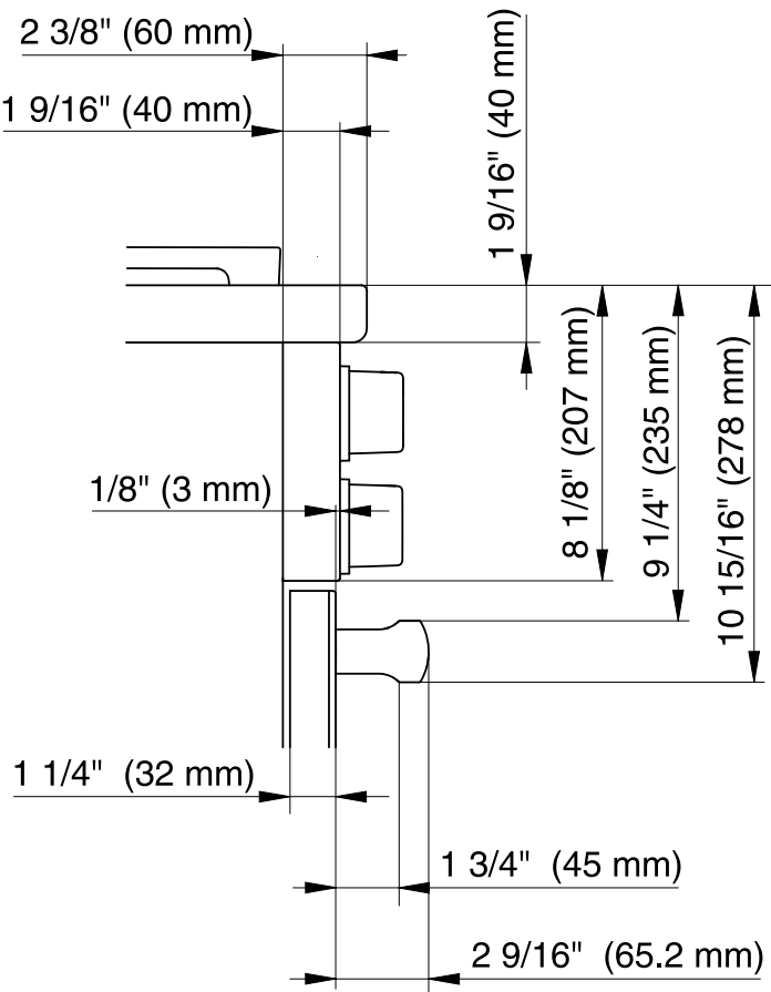
Detailed front side view of HR 1124-3 AG
