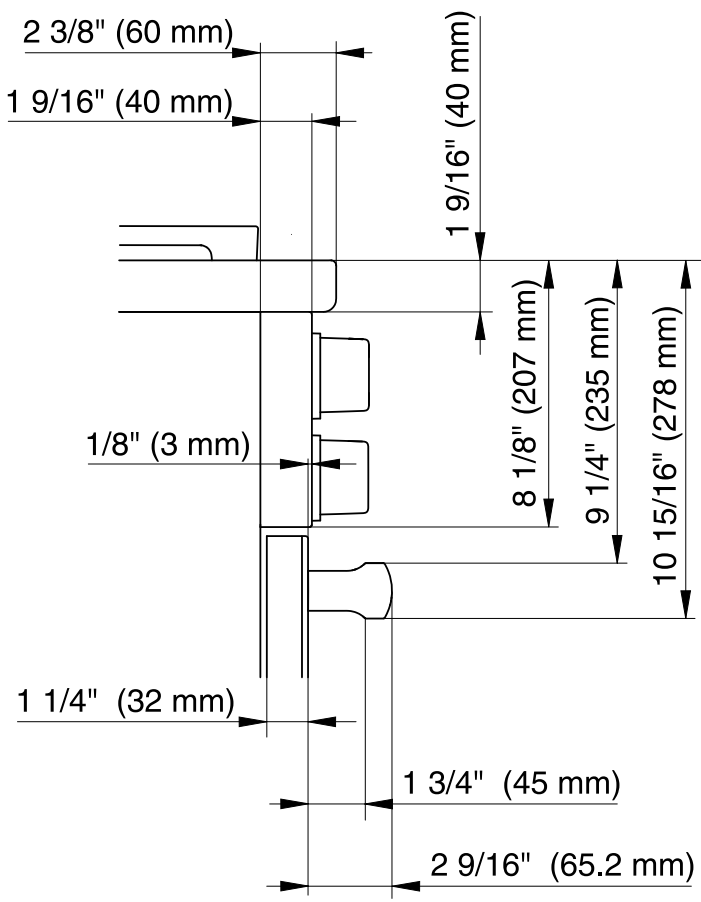
Detailed front side view of HR 1134-3 AG
