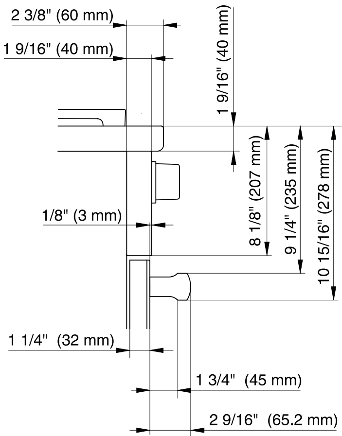
Detailed front side view of HR 1954-3 DF
