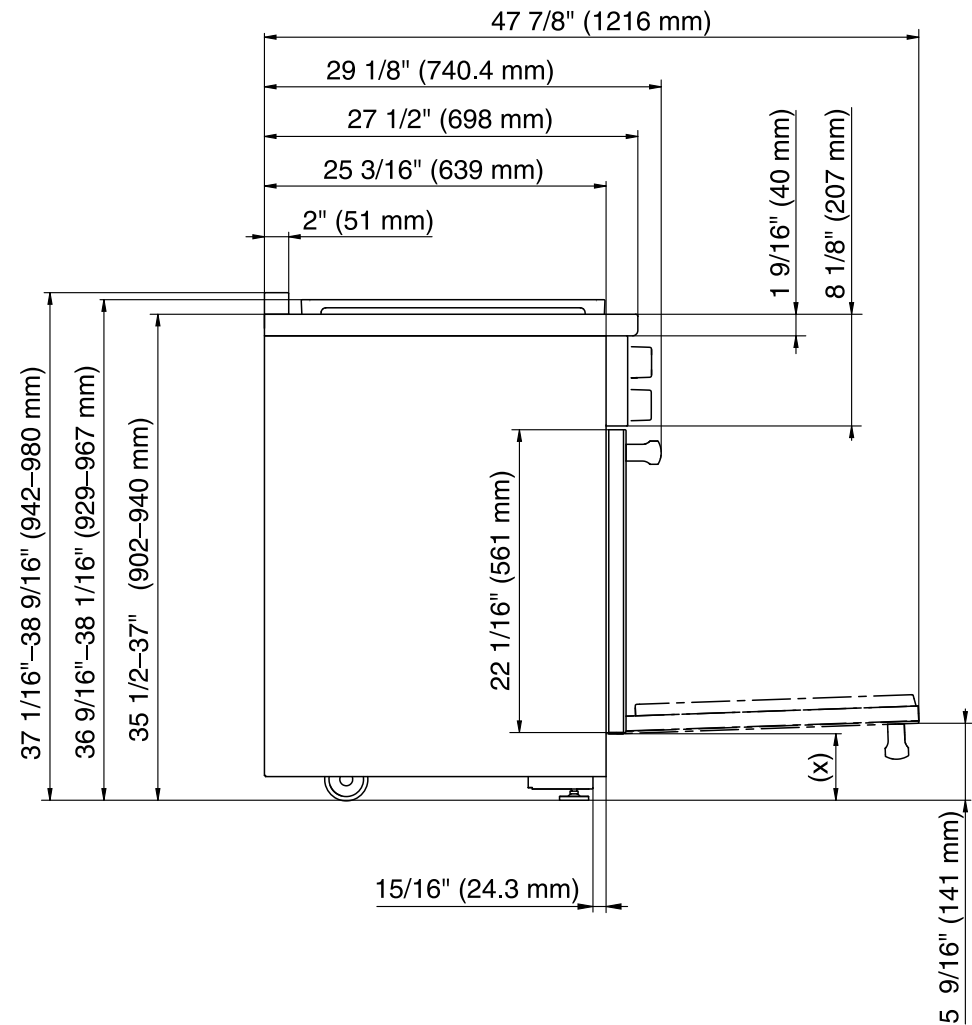
Side view of HR 1724-3 DF
