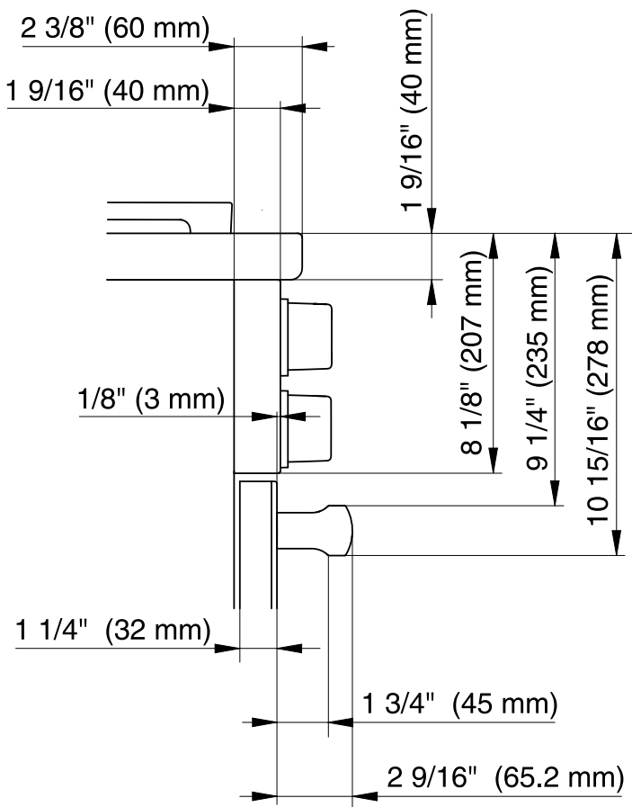
Detailed front side view of HR 1724-3 DF
