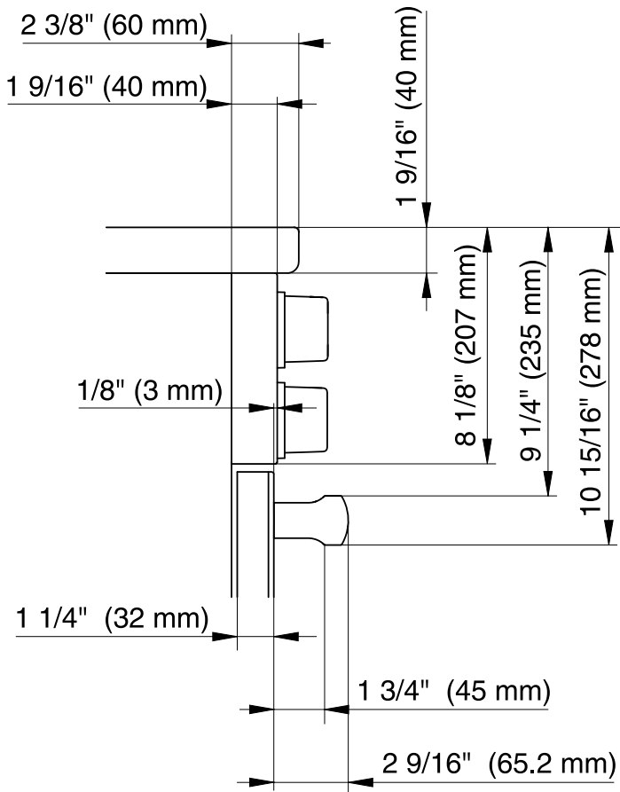
Detailed front side view of HR 1421-3 E
