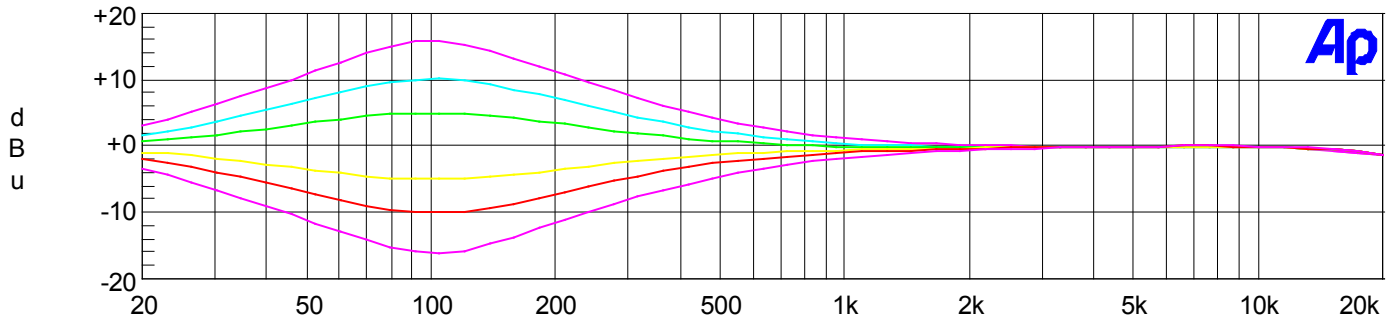
LF Shelf Button = Disabled, LF Frequency Center = 100 Hz, LF Q = Fully Counter-Clockwise, LF Gain = 5 dB Increments From 0 dBu
