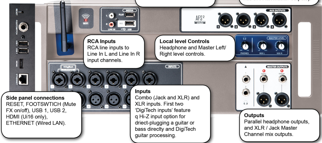
WiFi Antenna / LED WiFi access point to built-in web server enables browser-based software control.
