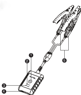
Figure 8-1 MaxiBAS BT506 Tester
