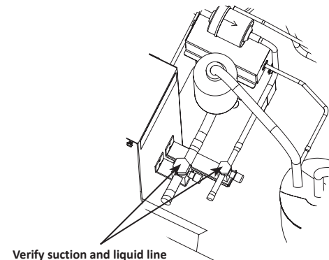
Verify suction and liquid line shut-off valves are open before operating the ice machine
