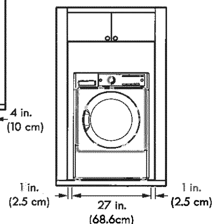
Standard Installation – Front View
