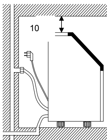
Side view (mm)
