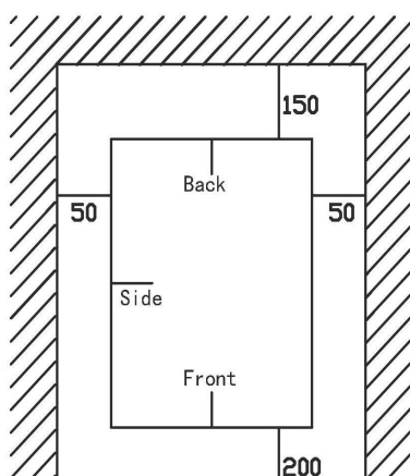
Installation clearance top view (mm)
