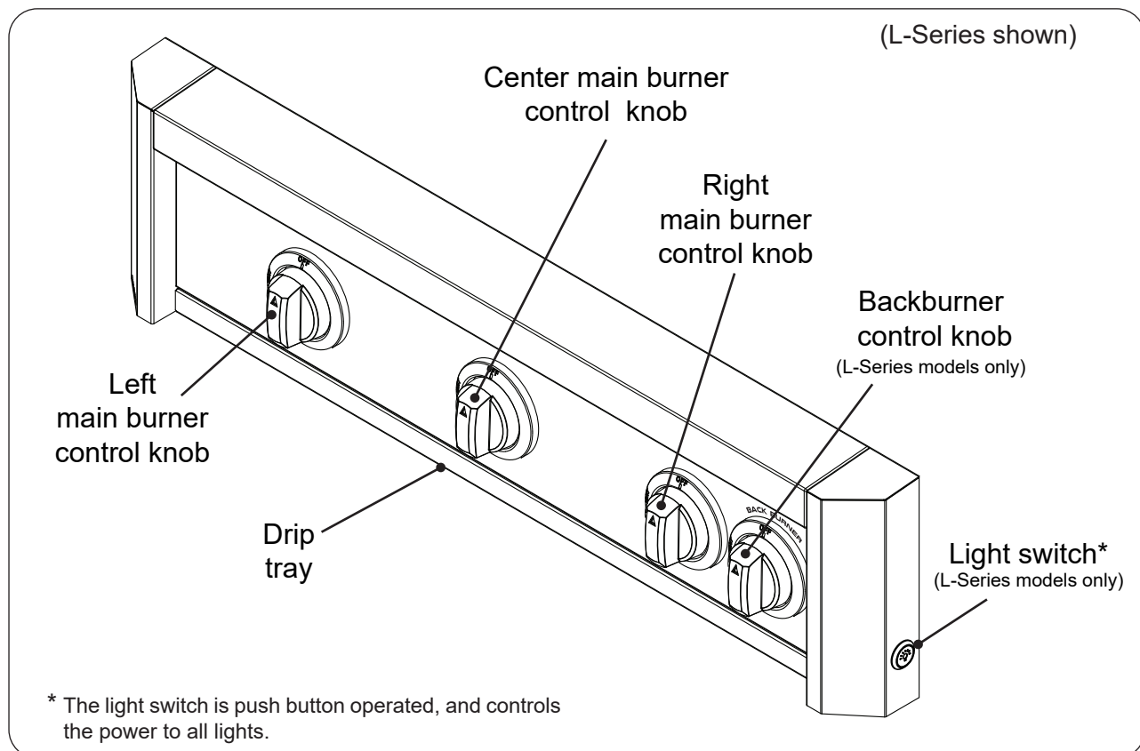
Fig. 31-2 30" and 36" model controls
