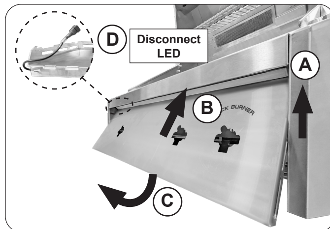
Fig. 40-3 Remove face panel
