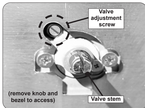
Fig. 45-1 Valve adjustment screw location
