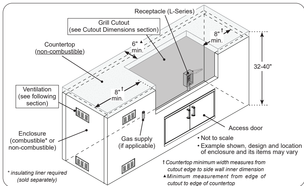
Fig. 11-1 Enclosure specifications
