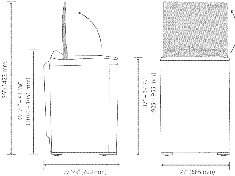
Fig.6 AeroSmart dimensions
