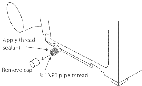
Fig.35 Preparing for gas tubing connection
