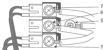
Fig.32 Connecting wiring
