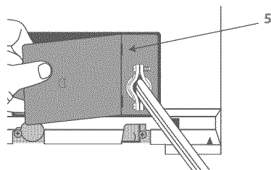
Fig.25 Refitting terminal block cover
