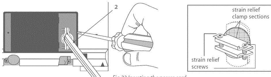
Fig.23 Inserting the power cord
