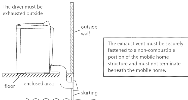
Fig.8 Exterior venting
