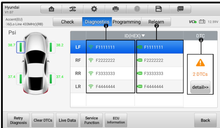
Figure 6-17 Diagnostics Screen 1
