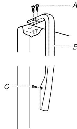
A. Flat-head handle screws B. Refrigerator door handle C. 1/4" Setscrew
