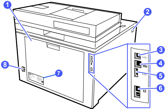
Figure 1-7 Printer rear view
