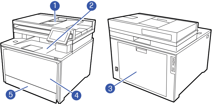
Figure 9-11 Jam locations
