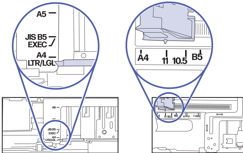
Figure 9-10 Size markings for cassette trays
