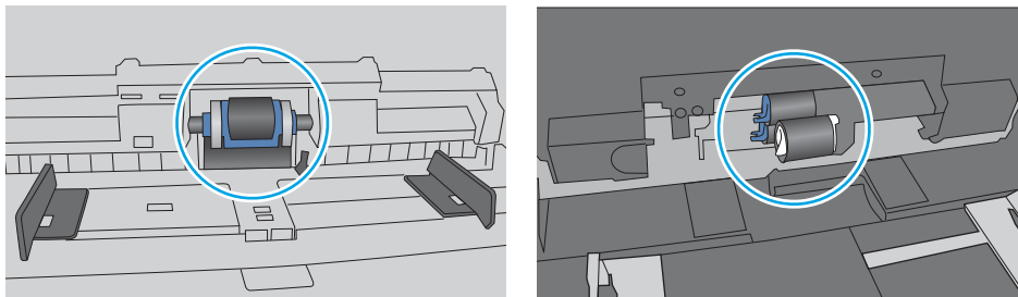
Figure 9-5 Roller locations for Tray 1 or the multipurpose tray
