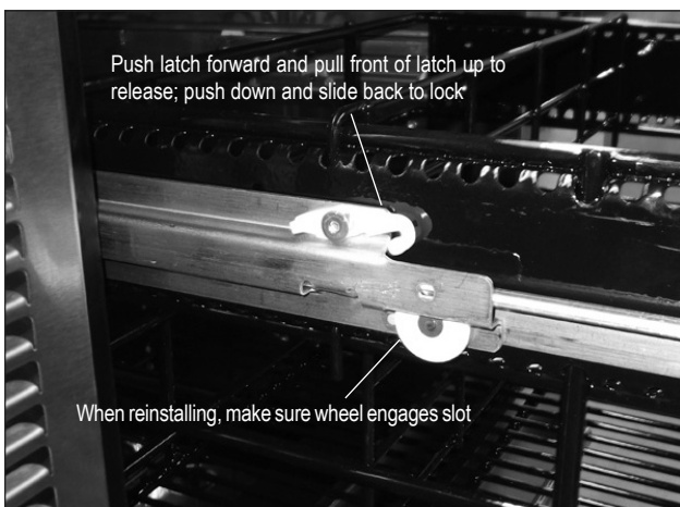
Figure 16: Removing/Installing Drawer
