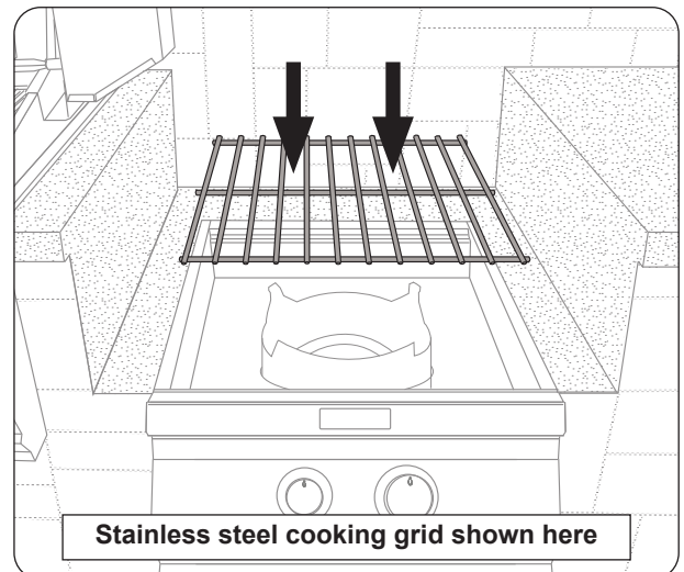
Fig. 27-4 Install cooking grid
