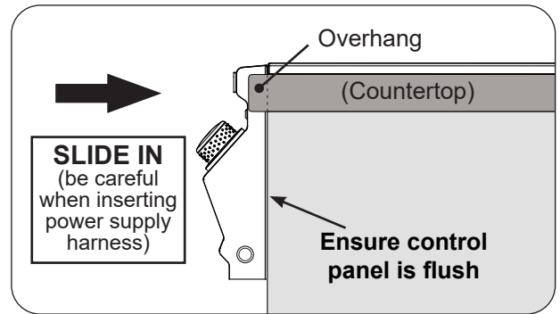
Fig. 27-1 Slide in unit (ensure flush)
