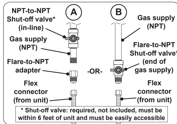
Fig. 28-1 Connecting to a gas line
