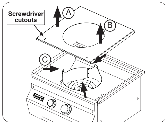
Fig. 40-1 Interior protection plate removal
