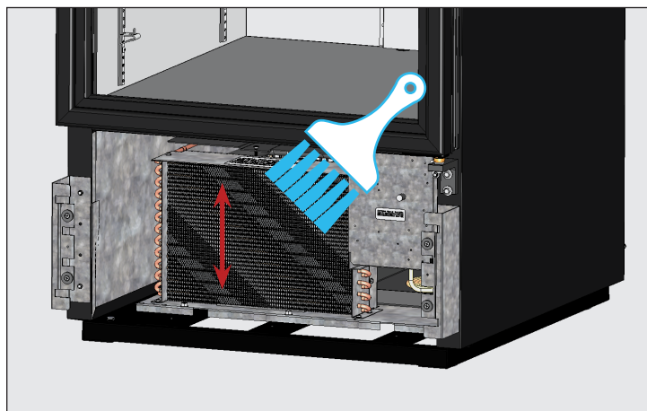
Fig. 4. Never brush across the coil fins.
