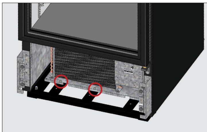
Fig. 6. Remove condenser base bolts.
