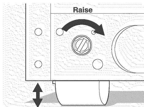
Adjustable Front Roller (some models)
