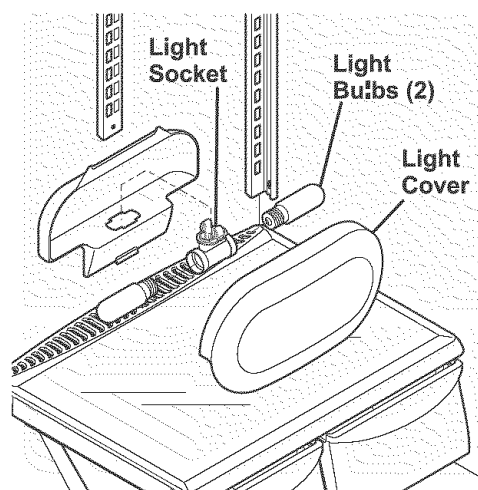
Refrigerator Mid-Level Light Cover Removal
