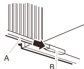
FIG.7C Bottom view
