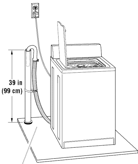
Standpipe drain system: Needs a 2 in (5 cm) minimum diameter standpipe with minimum carry-away capacity of 17 gal (64 L) per minute. Top of standpipe must be at least 39 in (99 cm) above floor and no higher than 96 in (2.4 m) from bottom of washer.
