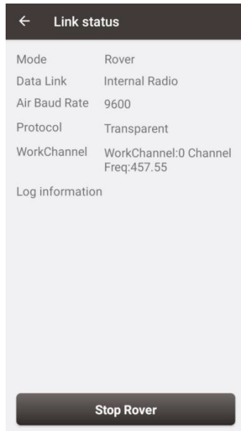
Figure 2.4 Internal Radio
