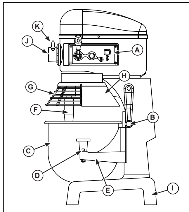
Figure 2. 20 Quart and 30 Quart Mixers, Features and Controls.
