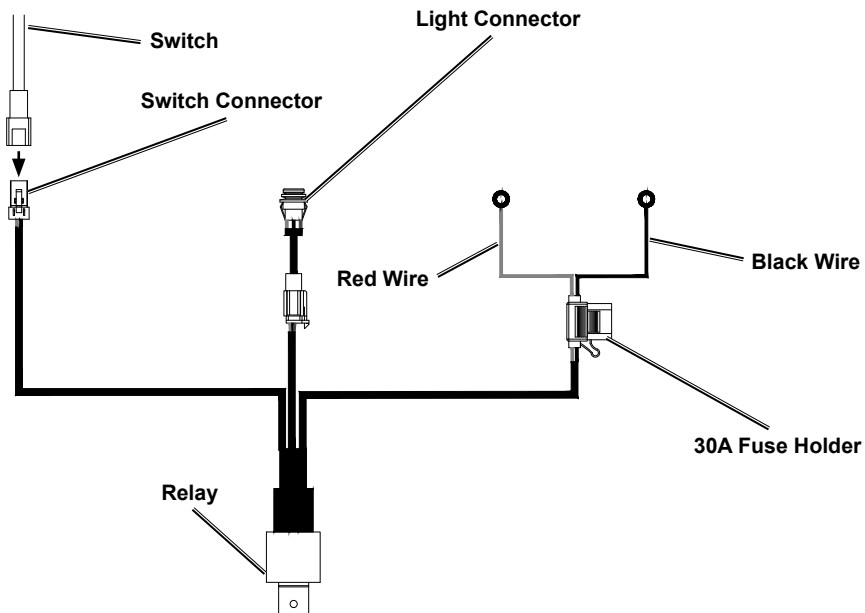
Figure B: Wiring Harness Connections
