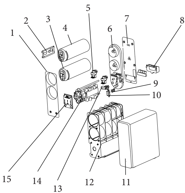
Explosion drawing of parts
