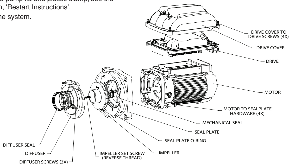
Motor Assembly
