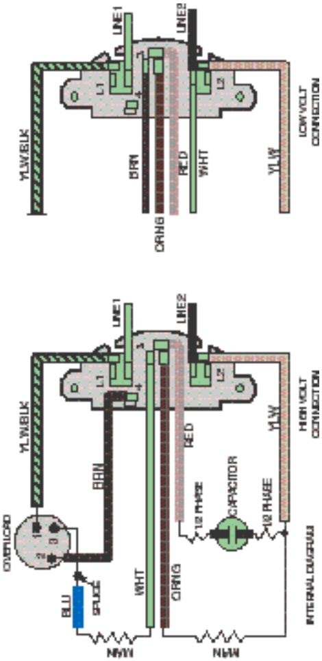
Wiring Diagram #166359. Connection Label #166362.
