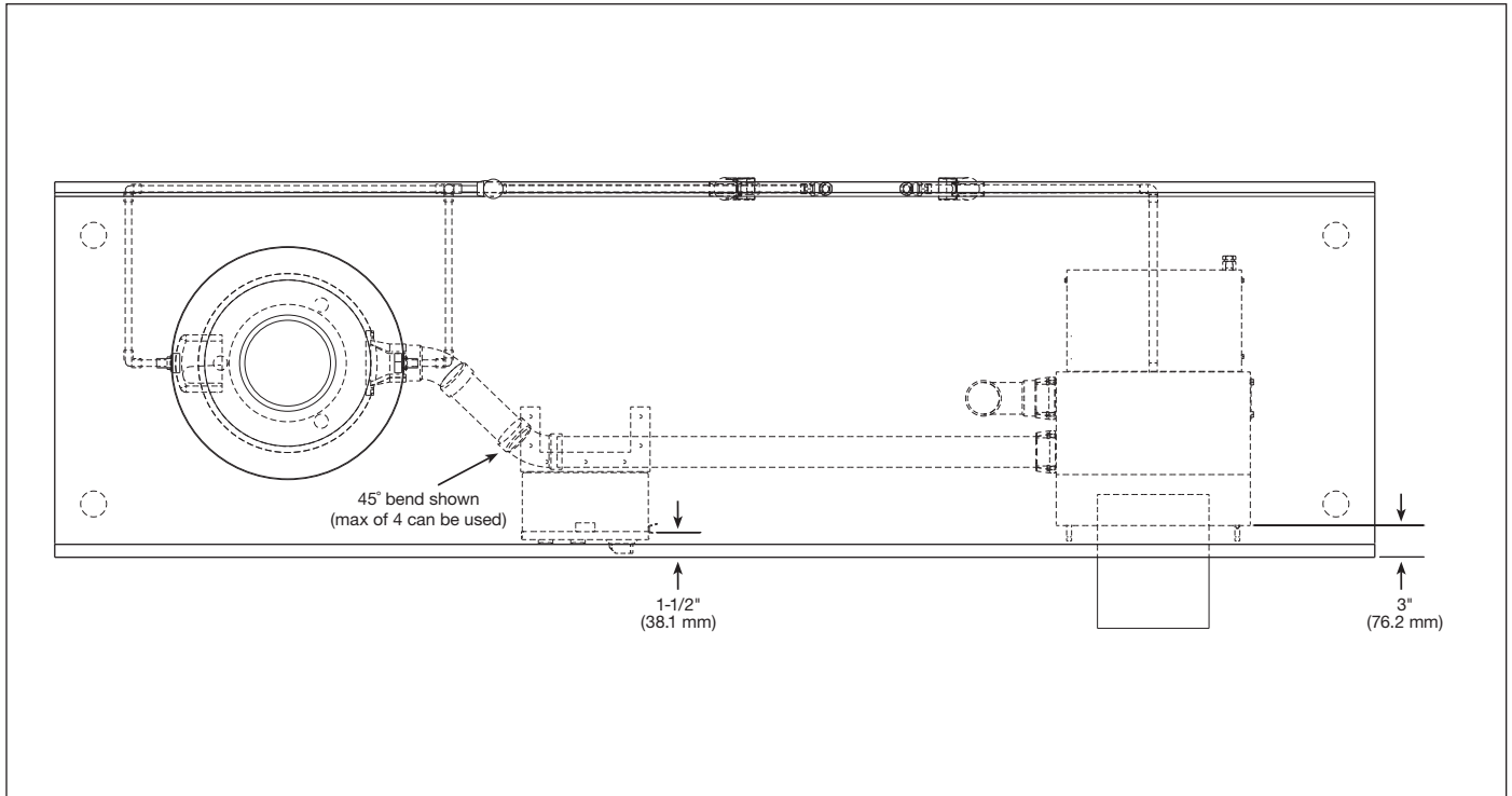
Figure 11. Top View
