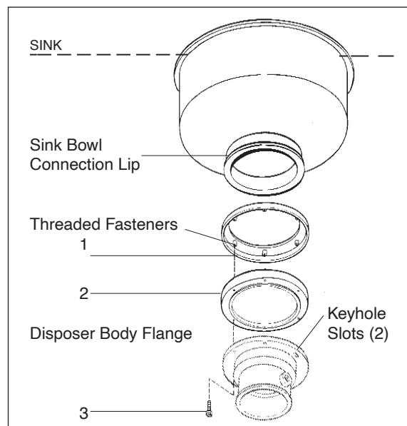
Figure 6. Adaptor Assembly with Disposer.
